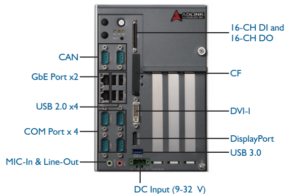
■ MXC-2300 Series Front Panel
